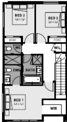
First Floor
