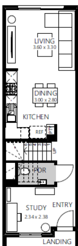
Ground Floor
