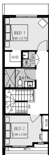
First Floor
